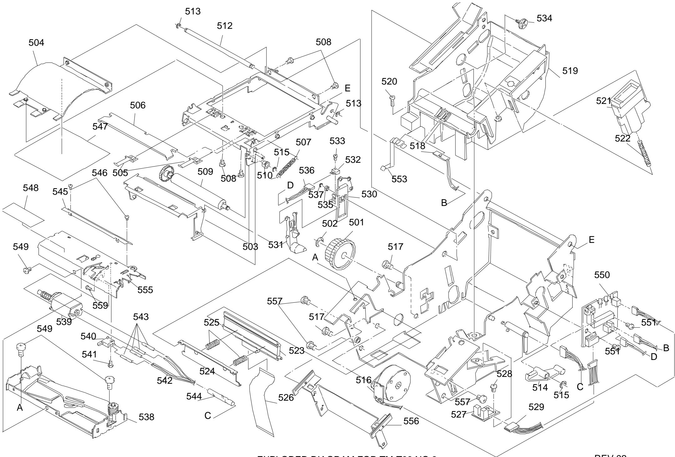
EXPLODED DIAGRAM FOR TM-T88 NO.2
