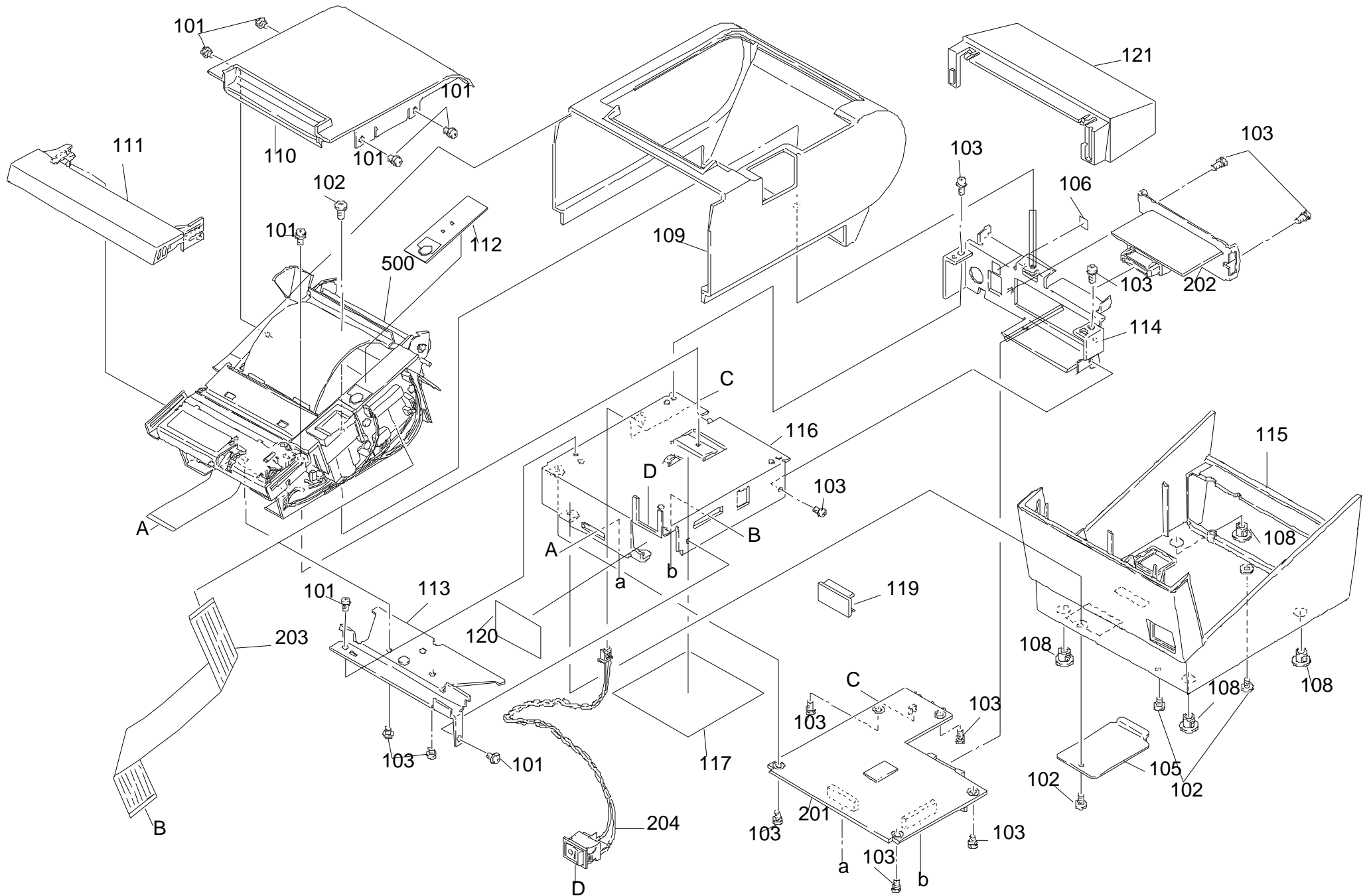
EXPLODED DIAGRAM FOR TM-T88 NO.1
