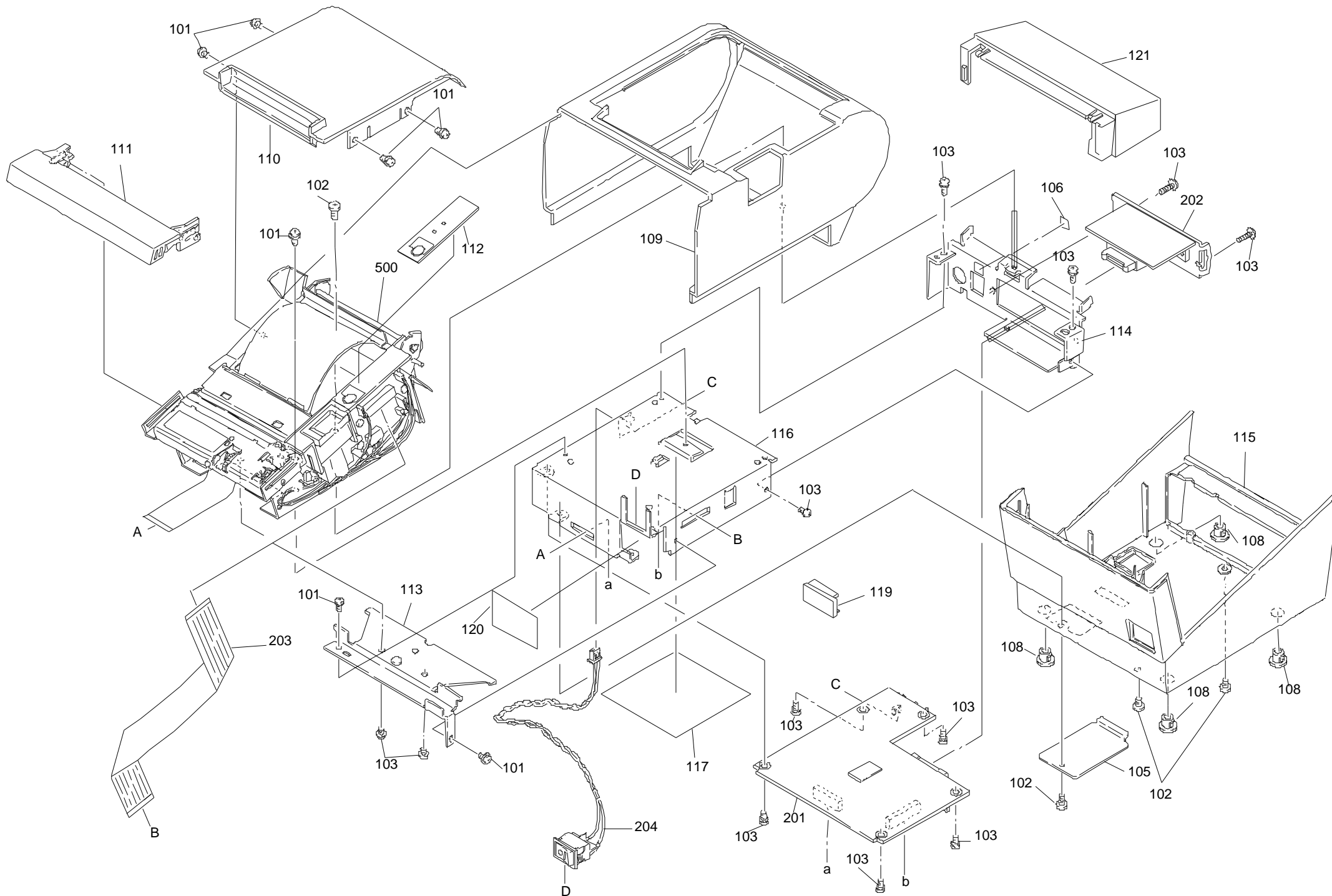
EXPLODED DIAGRAM FOR TM-T88IIP NO.1
