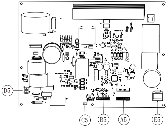
(#596 SUB-X #1 BOARD HOME SIDE )
