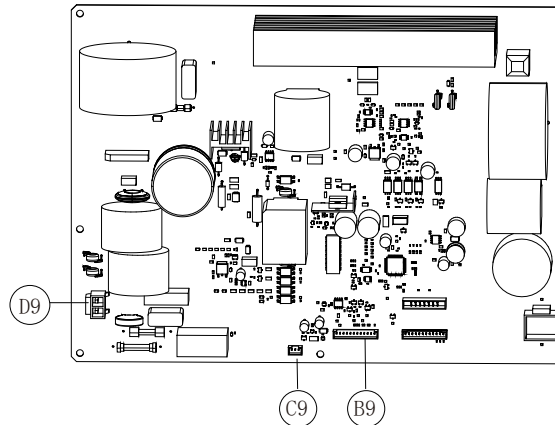
(#560 SUB-X #7 BOARD FULL SIDE RIGHT )
