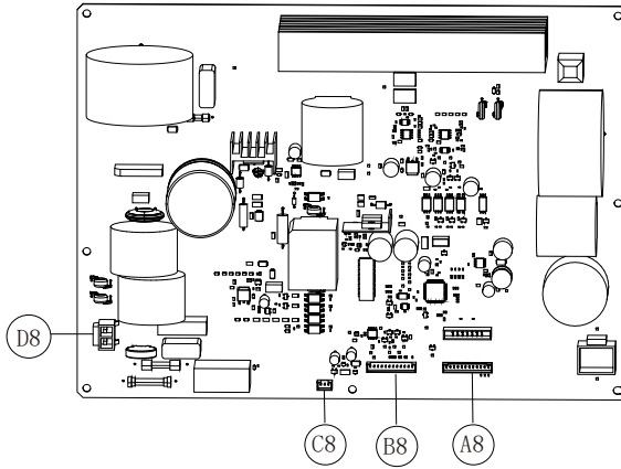
(#560 SUB-X #6 BOARD FULL SIDE LEFT )
