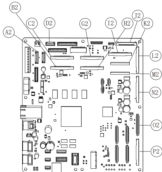
(#210 BOARD ASSY., MAIN)
