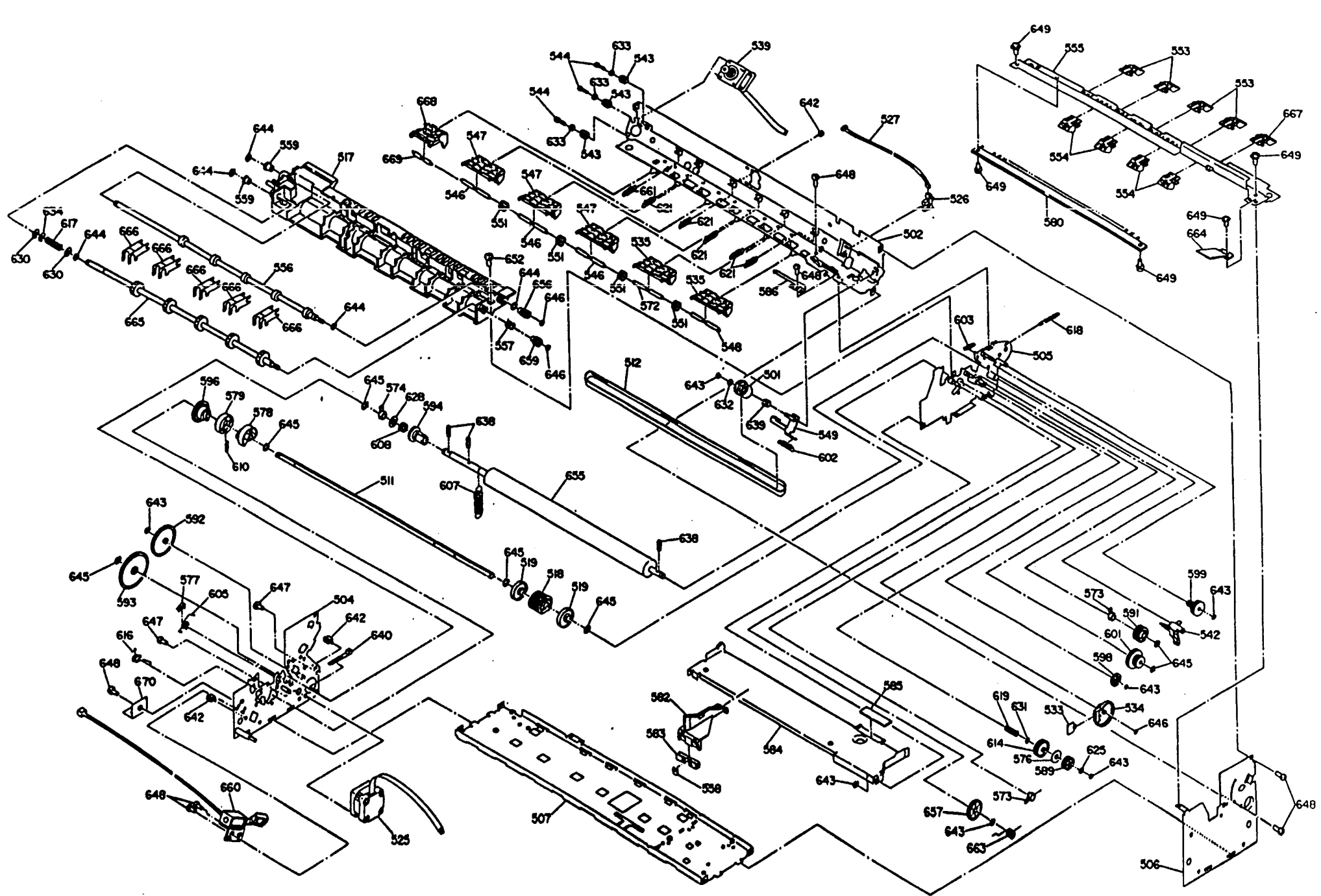
EXPLODED DIAGRAM FOR STYLUS PRO XL+(2)
