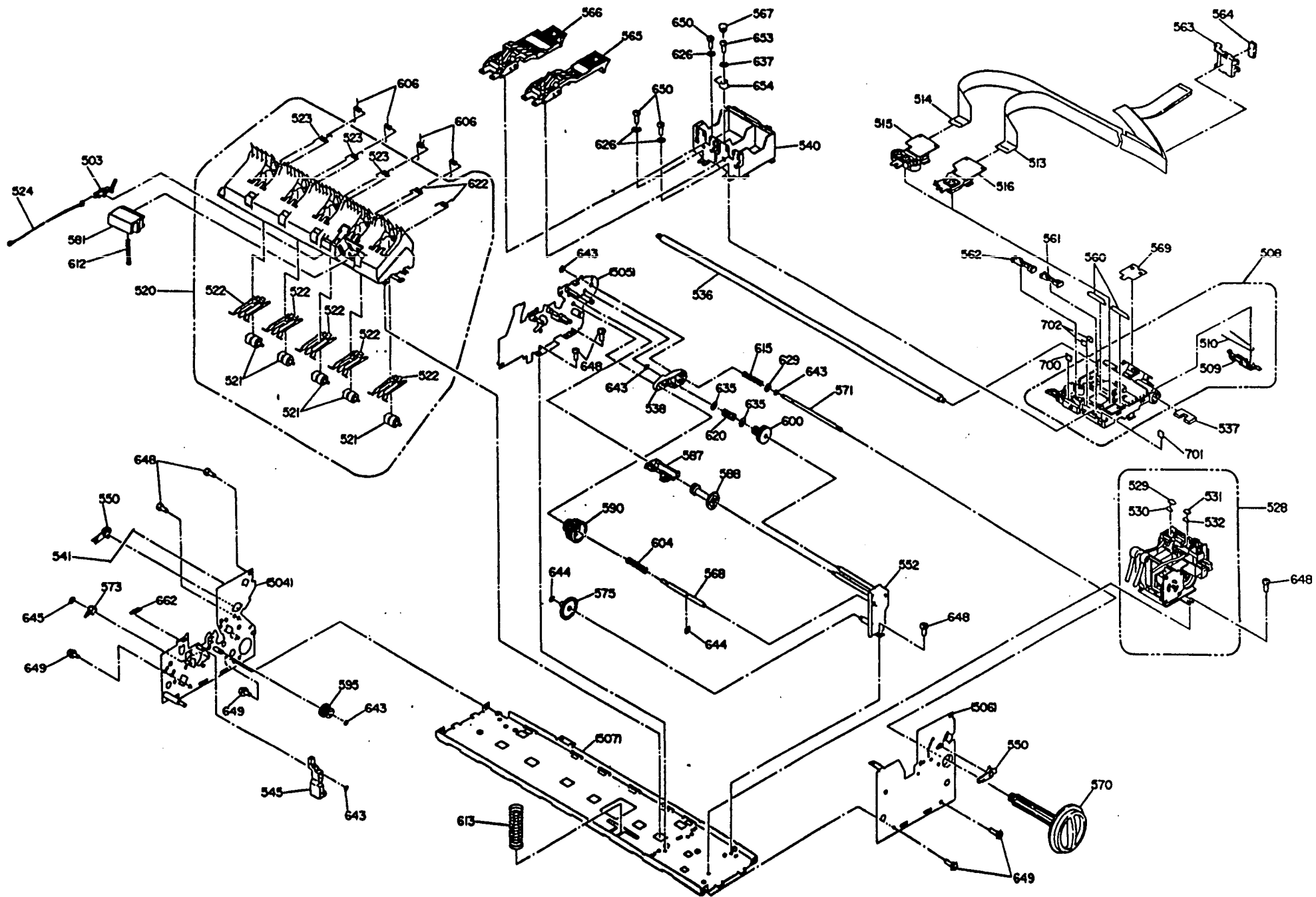
EXPLODED DIAGRAM FOR STYLUS PRO XL+(3)
