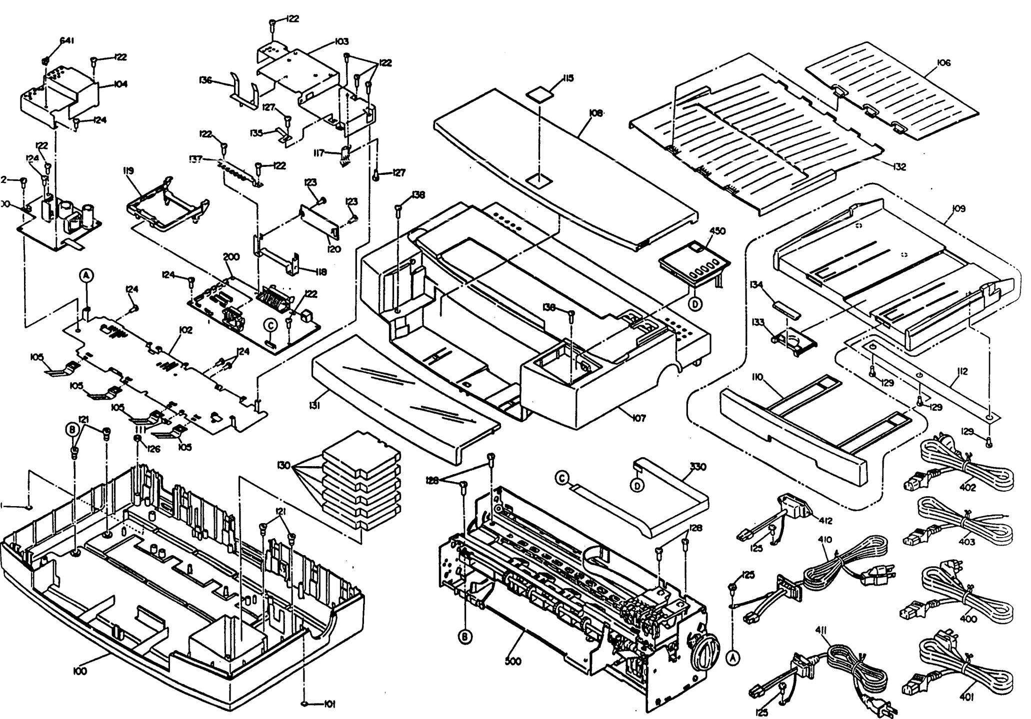
EXPLODED DIAGRAM FOR STYLUS PRO XL+(1)
