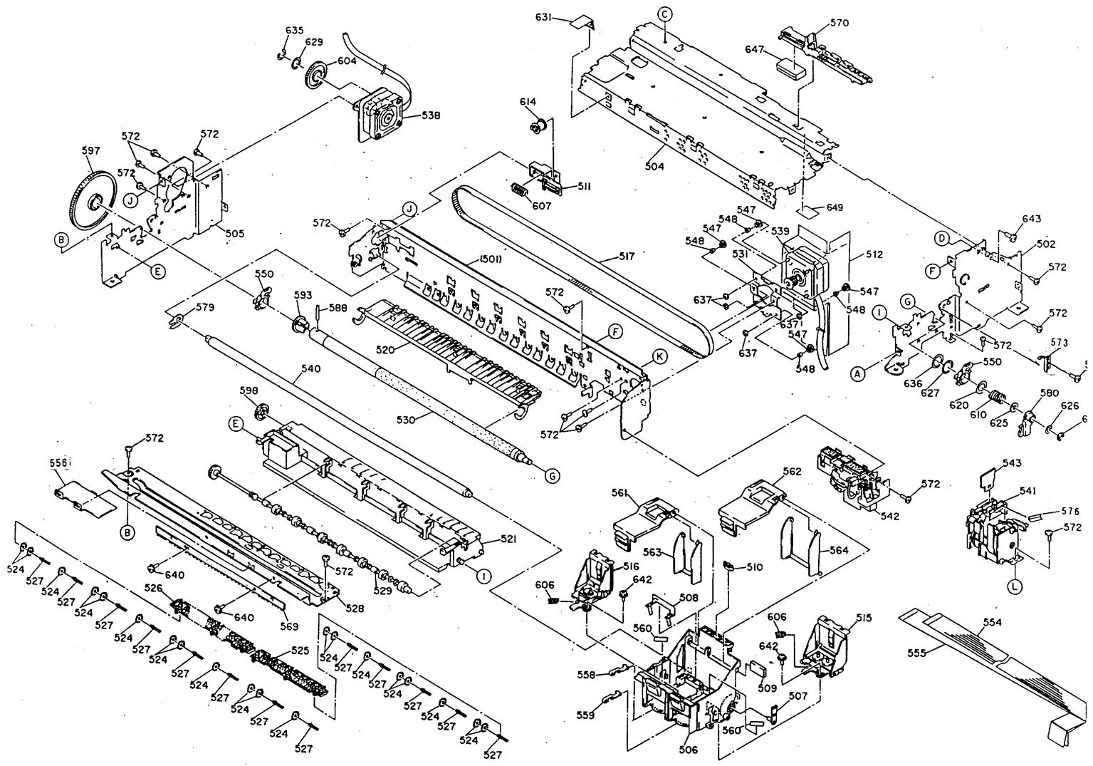
EXPLODED DIAGRAM FOR EPSON Stylus COLOR 850 (3/3)
