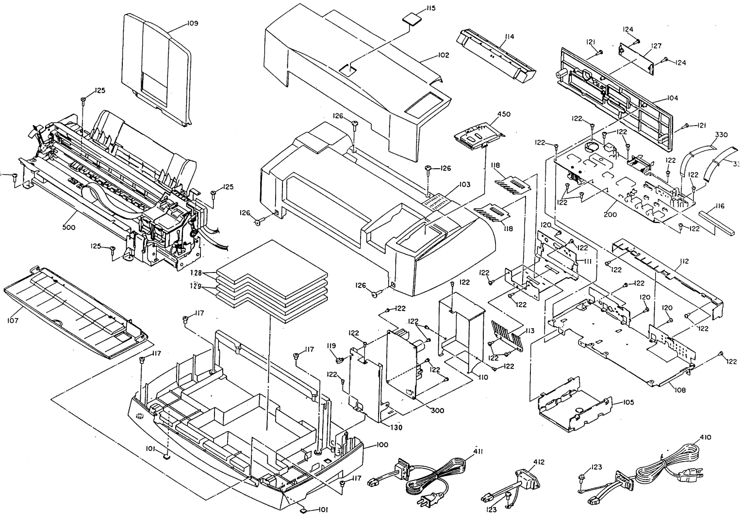
EXPLODED DIAGRAM FOR EPSON Stylus COLOR 850 (1/3)
