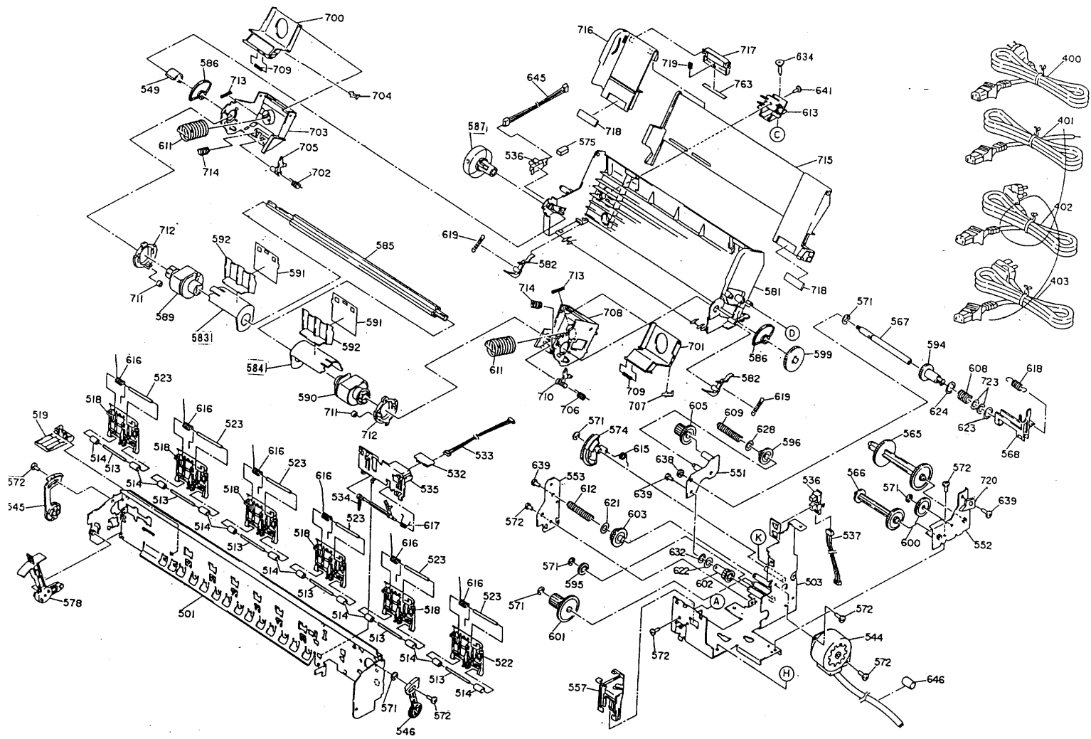
EXPLODED DIAGRAM FOR EPSON Stylus COLOR 850 (2/3)
