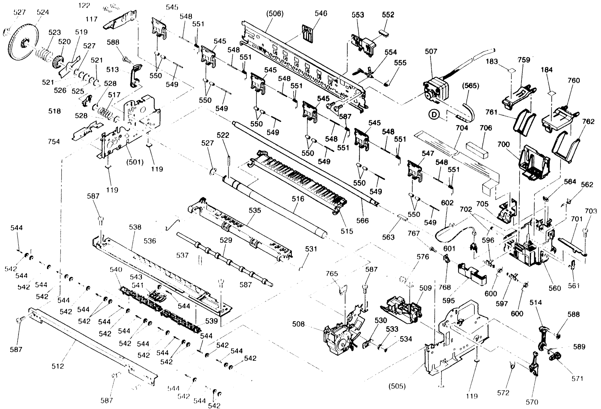
EXPLODED DIAGRAM FOR EPSON STYLUS COLOR 740 (3/3)
