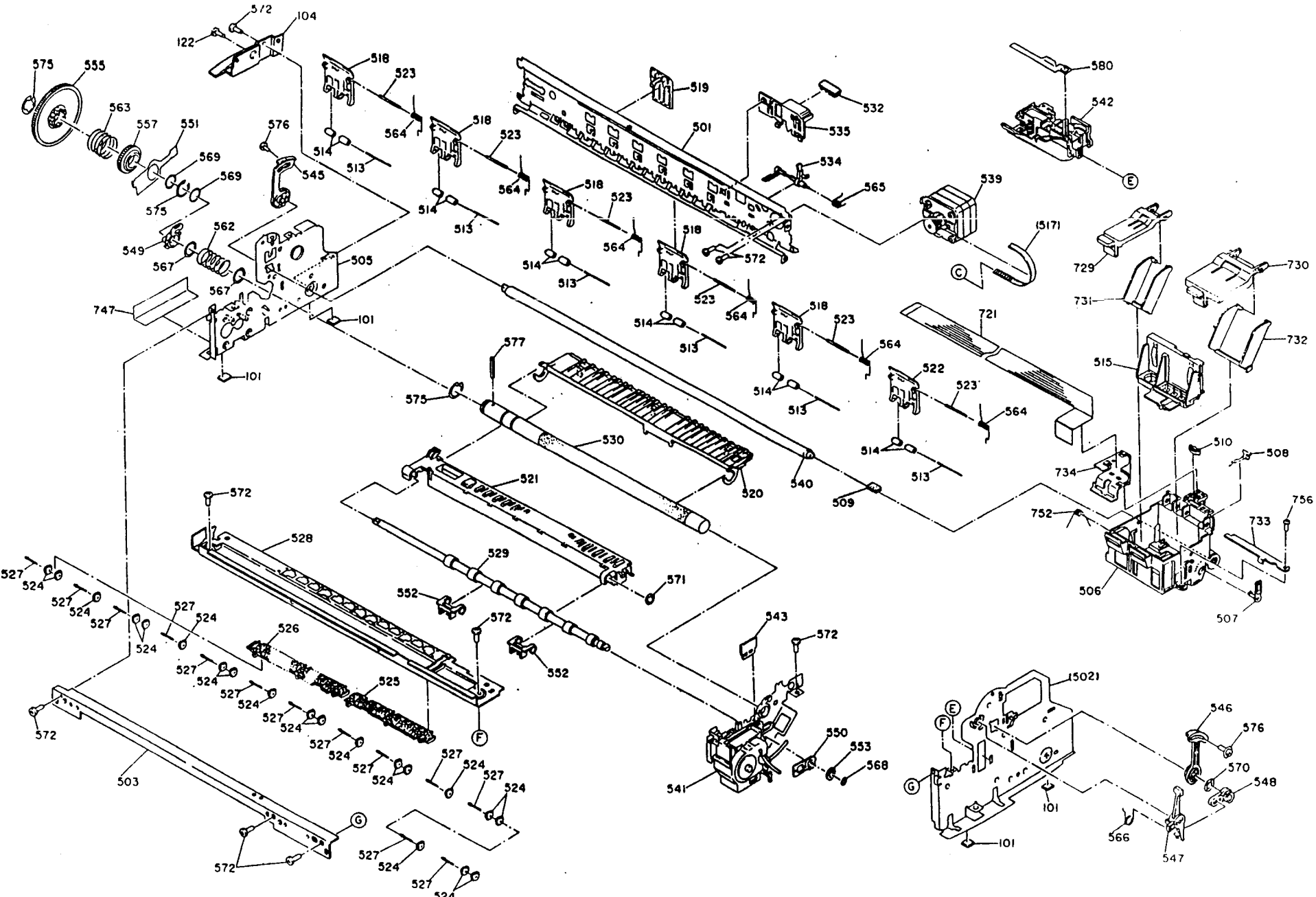
EXPLODED DIAGRAM FOR STYLUS COLOR 600 Compaq (3)
