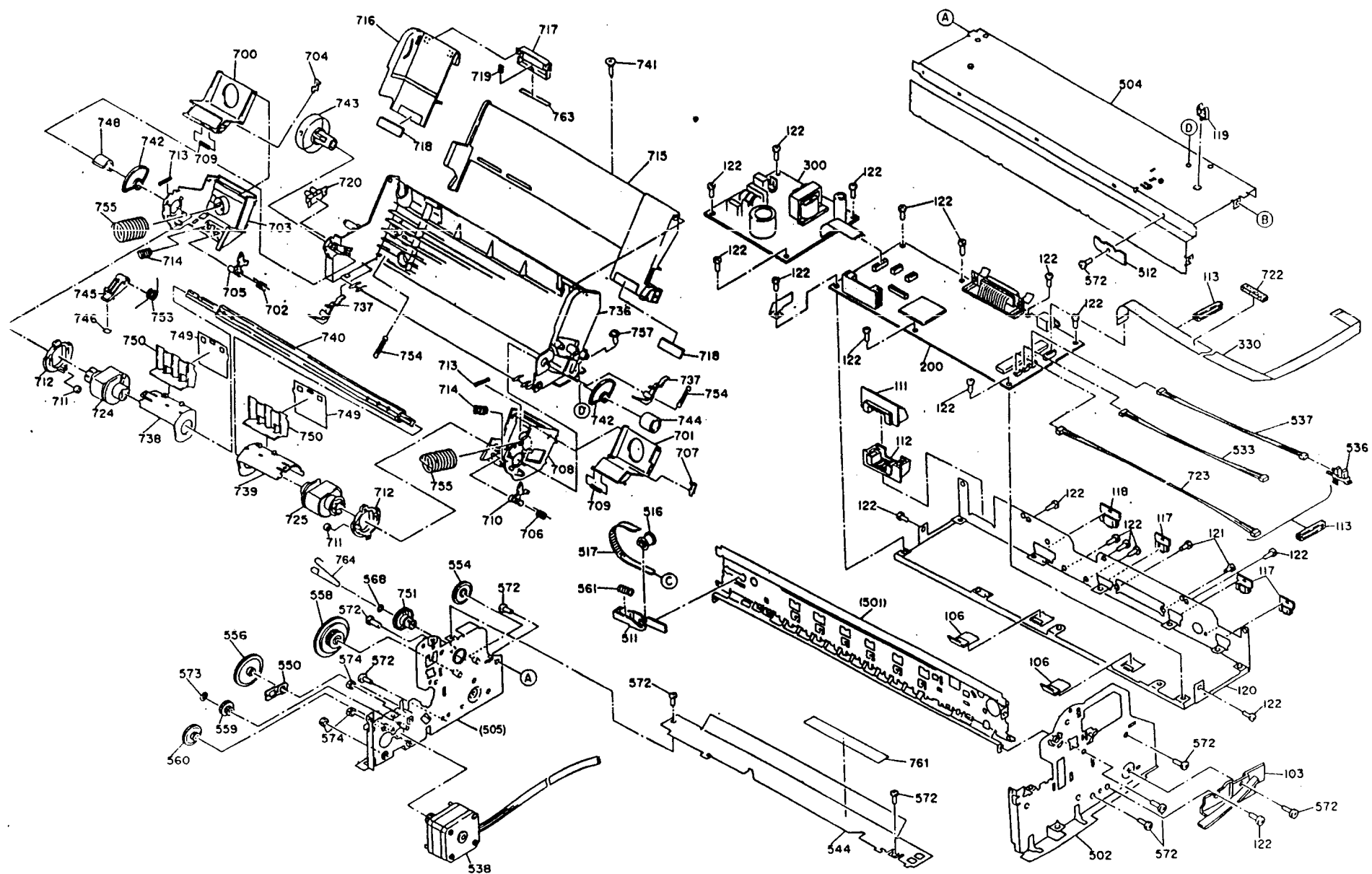
EXPLODED DIAGRAM FOR STYLUS COLOR 600 Compaq (2)
