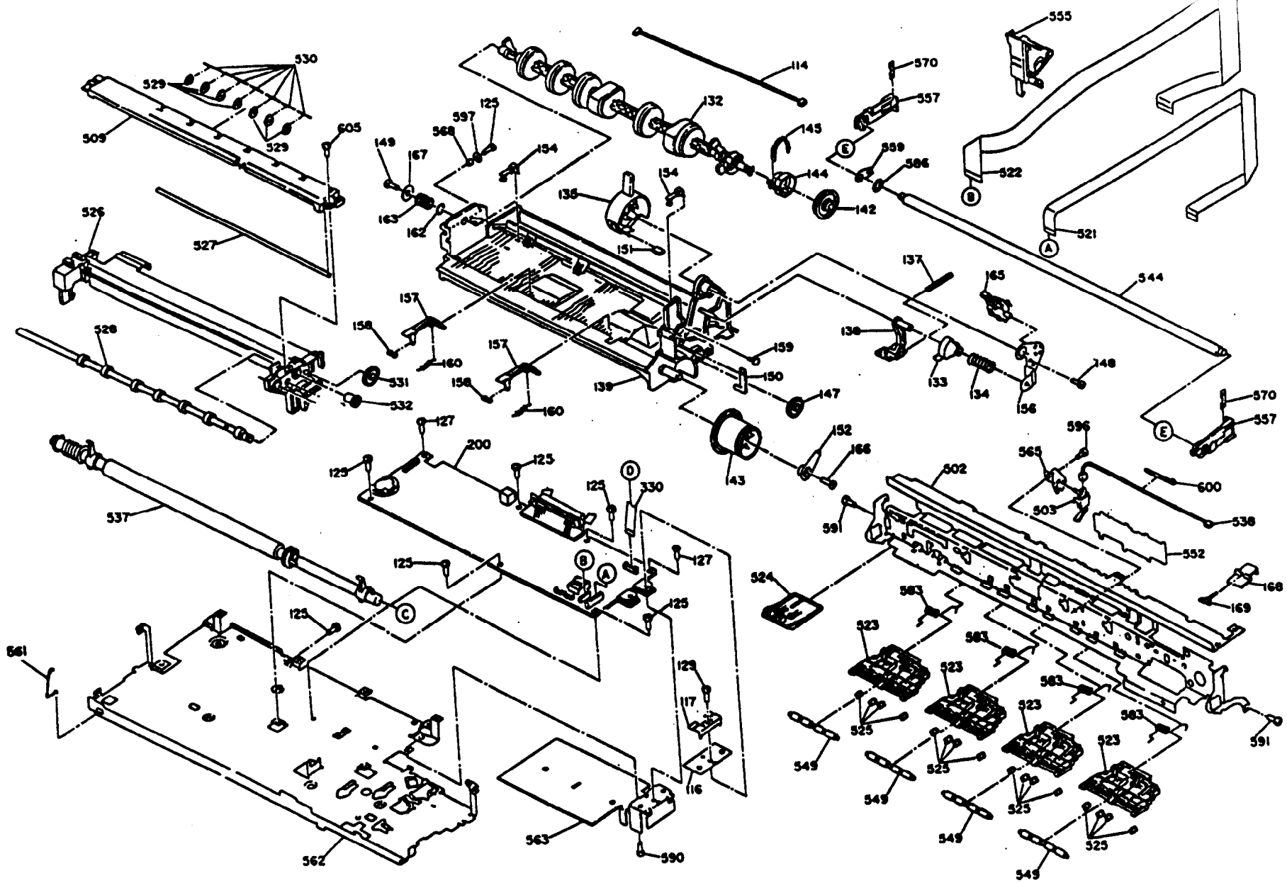
EXPLODED DIAGRAM FOR STYLUS COLOR 500(2)
