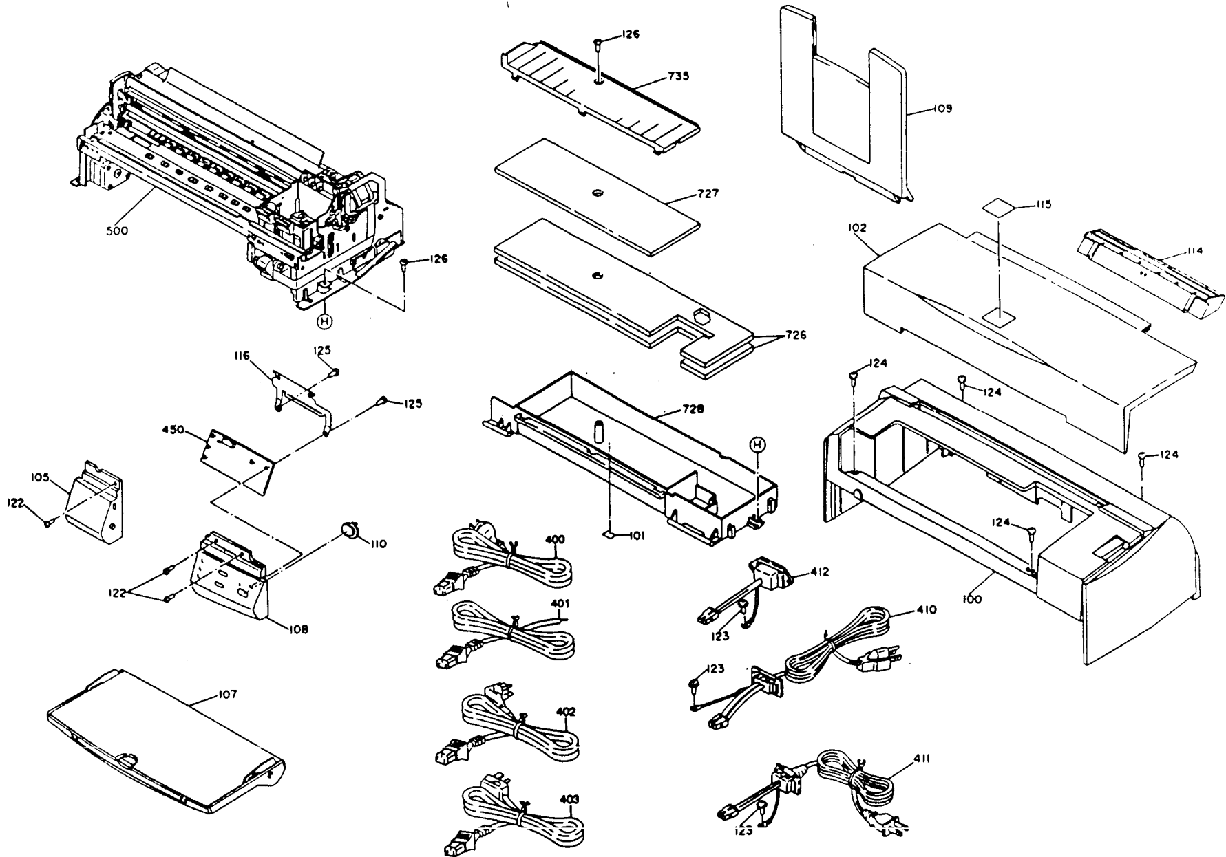
EXPLODED DIAGRAM FOR STYLUS COLOR 400 (I)
