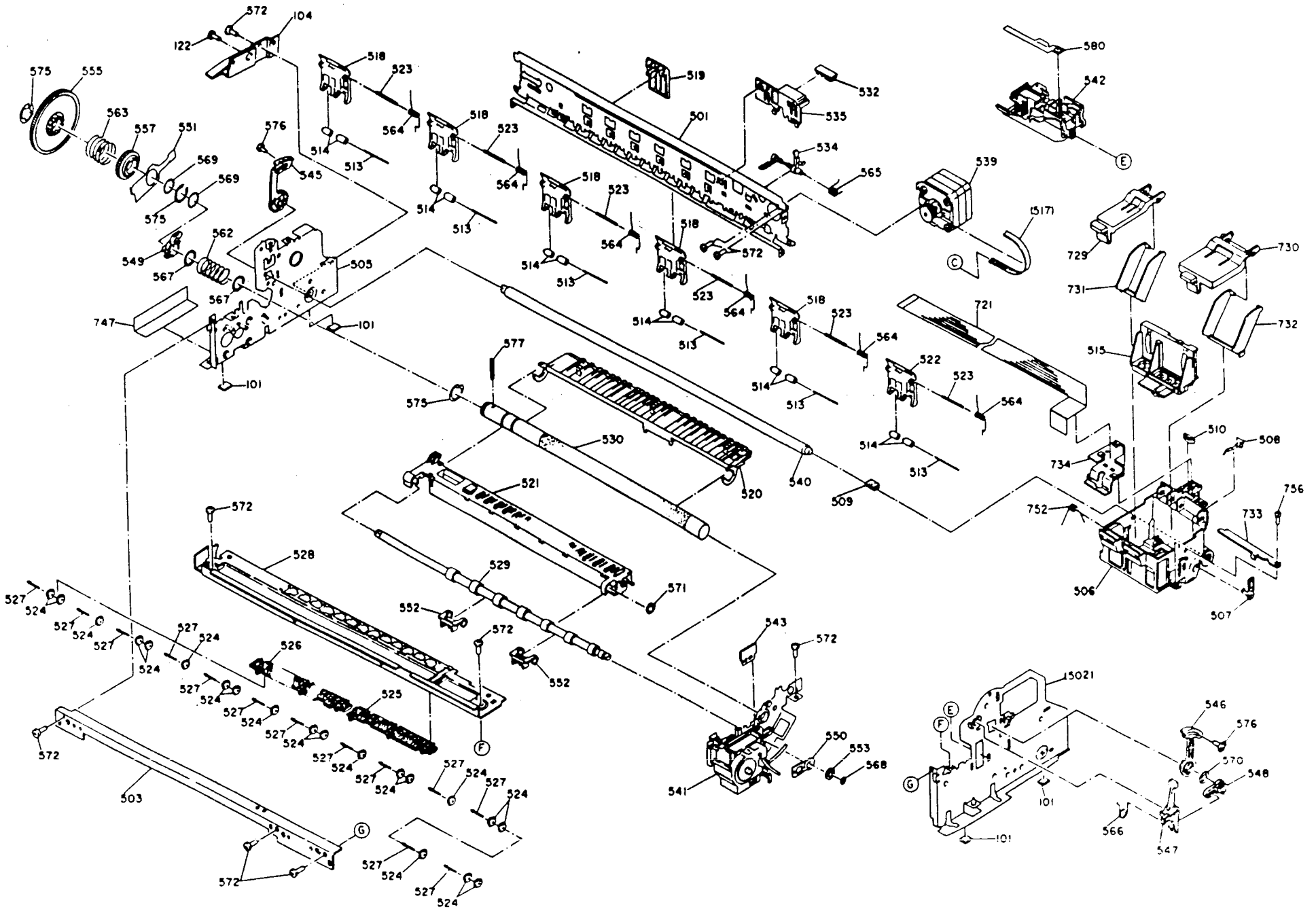
EXPLODED DIAGRAM FOR STYLUS COLOR 400 (3)
