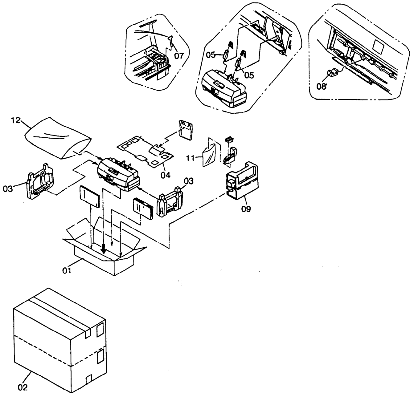
PACKING MATERIAL FOR STYLUS COLOR 200
