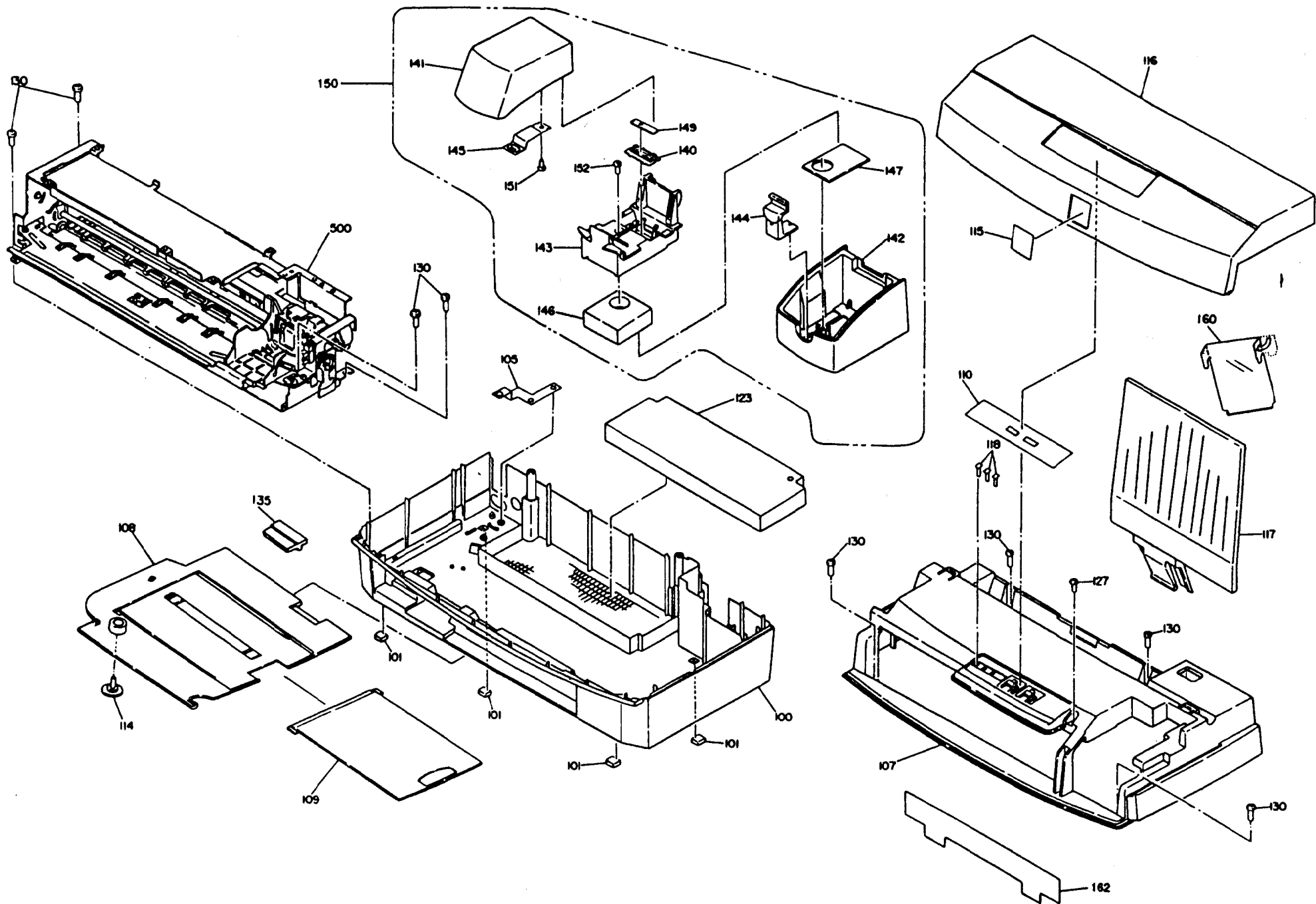
EXPLODED DIAGRAM FOR STYLUS COLOR 200(1)
