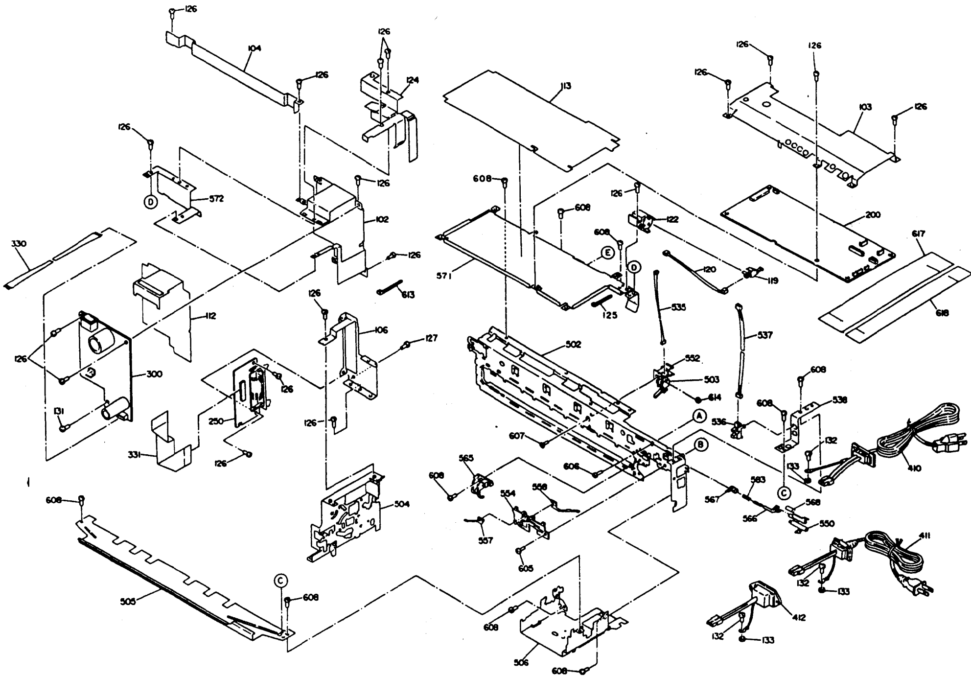
EXPLODED DIAGRAM FOR STYLUS COLOR 200(2)
