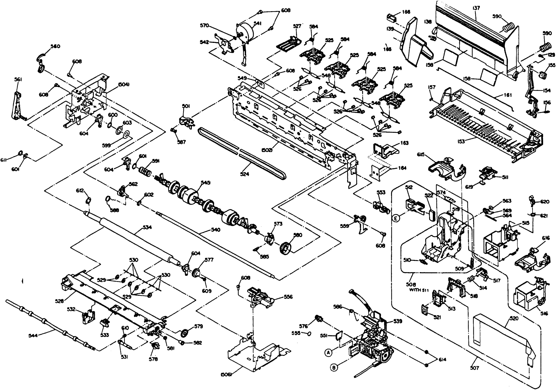
EXPLODED DIAGRAM FOR STYLUS COLOR 200(3)
