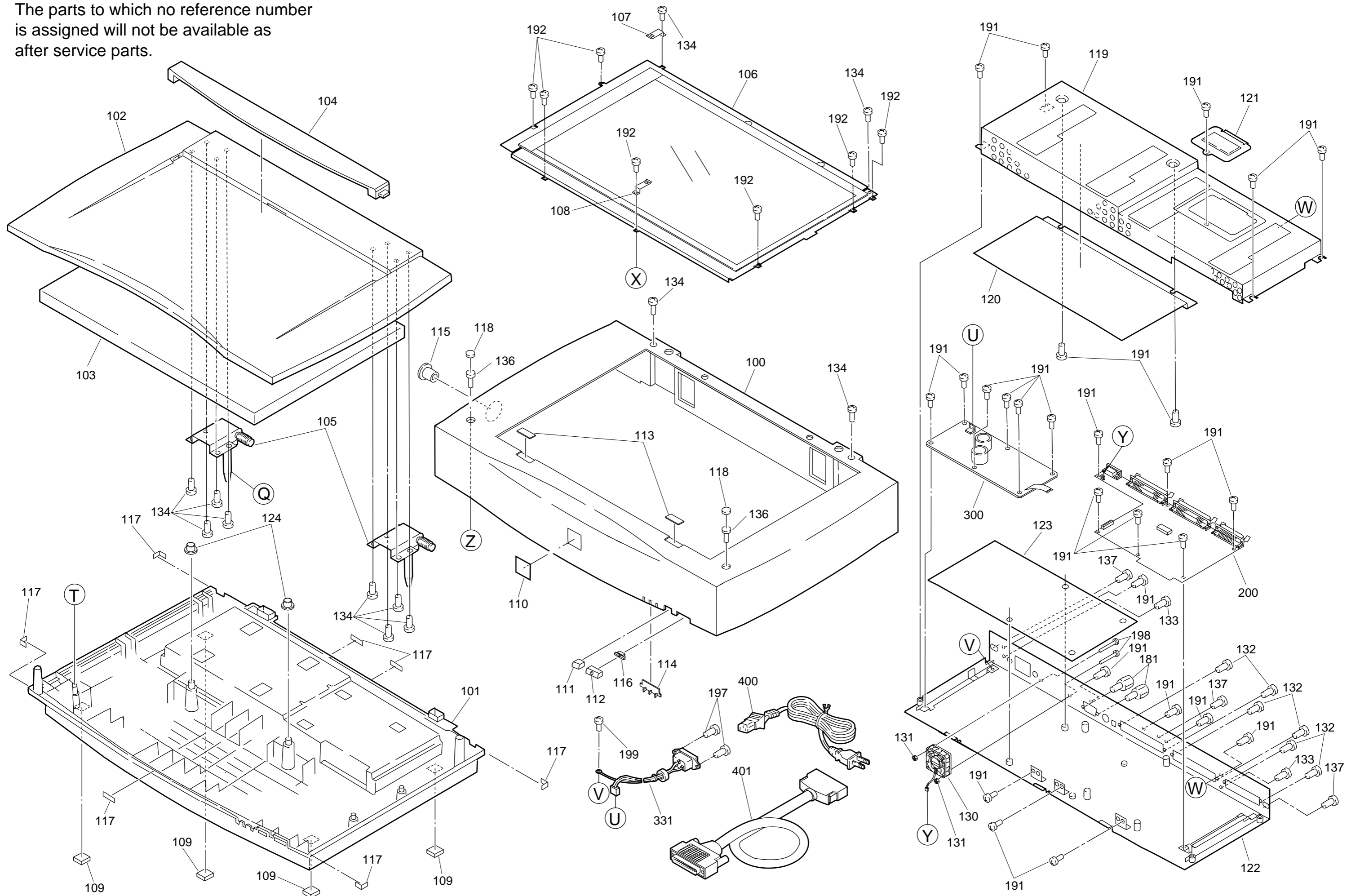
EXPLODED DIAGRAM FOR GT-12000 / Expression 836 (1)
