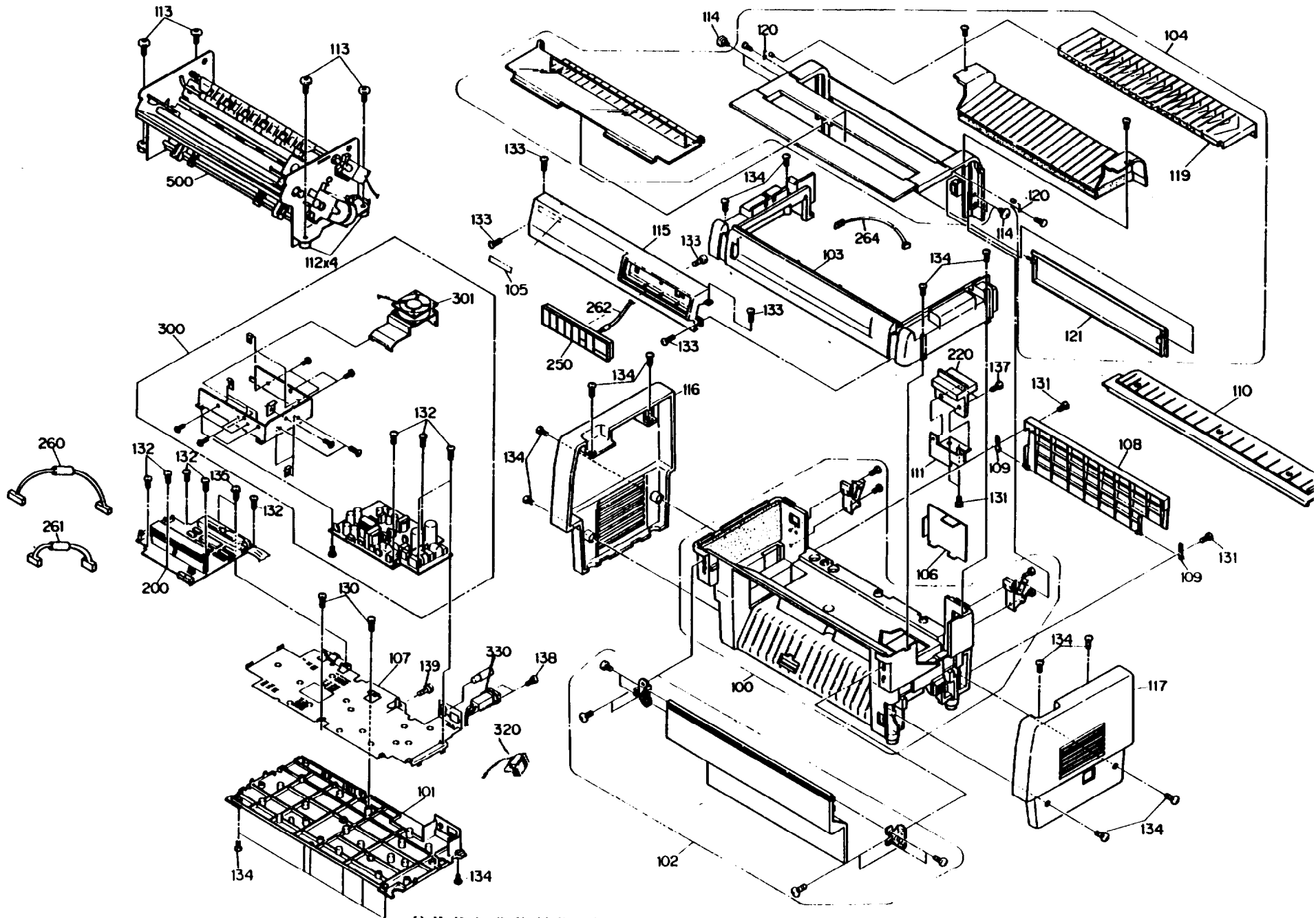
EXPLODED DIAGRAM FOR BOX 5000 (1)
