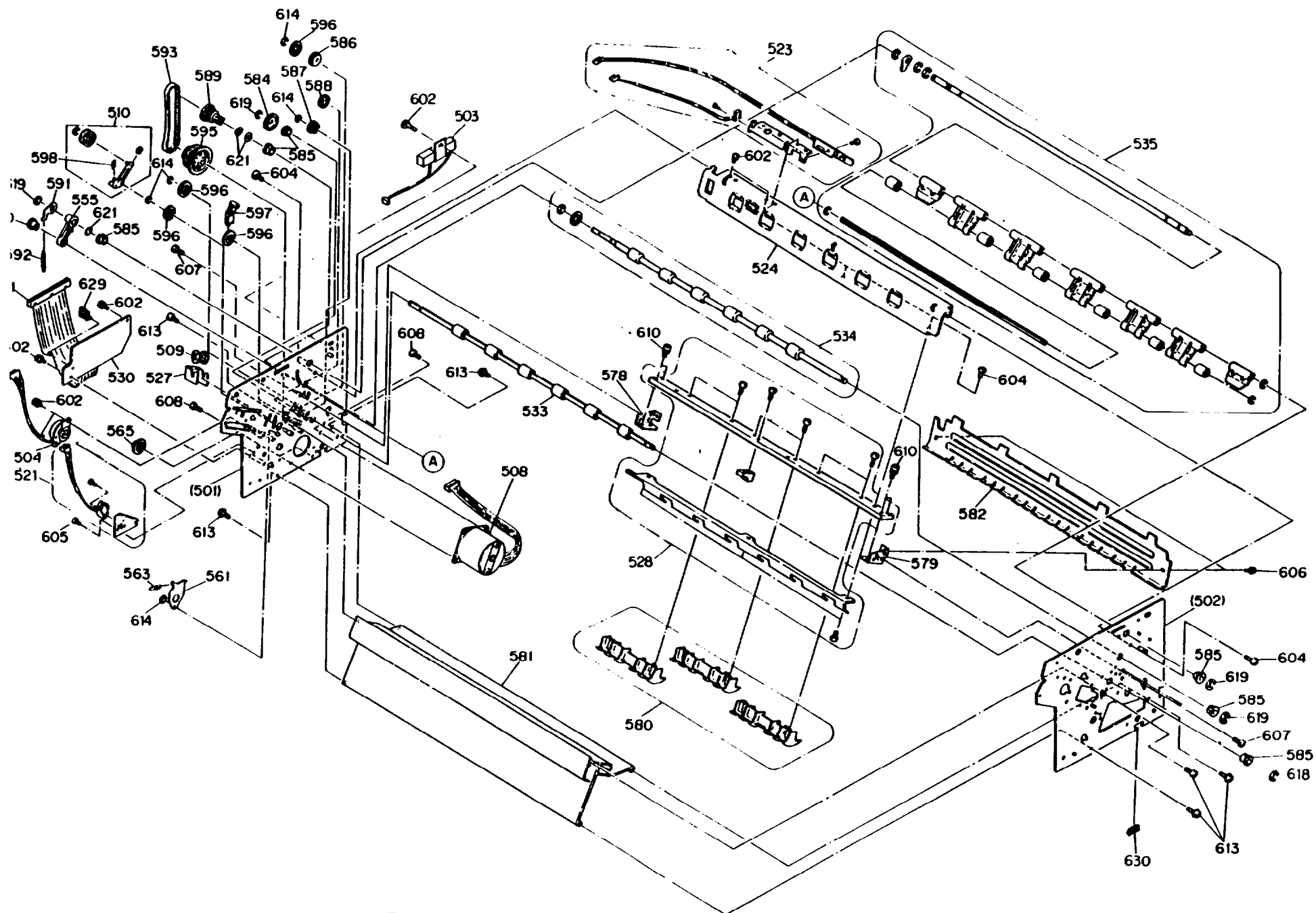
EXPLODED DIAGRAM FOR DFX-5000 (3)
